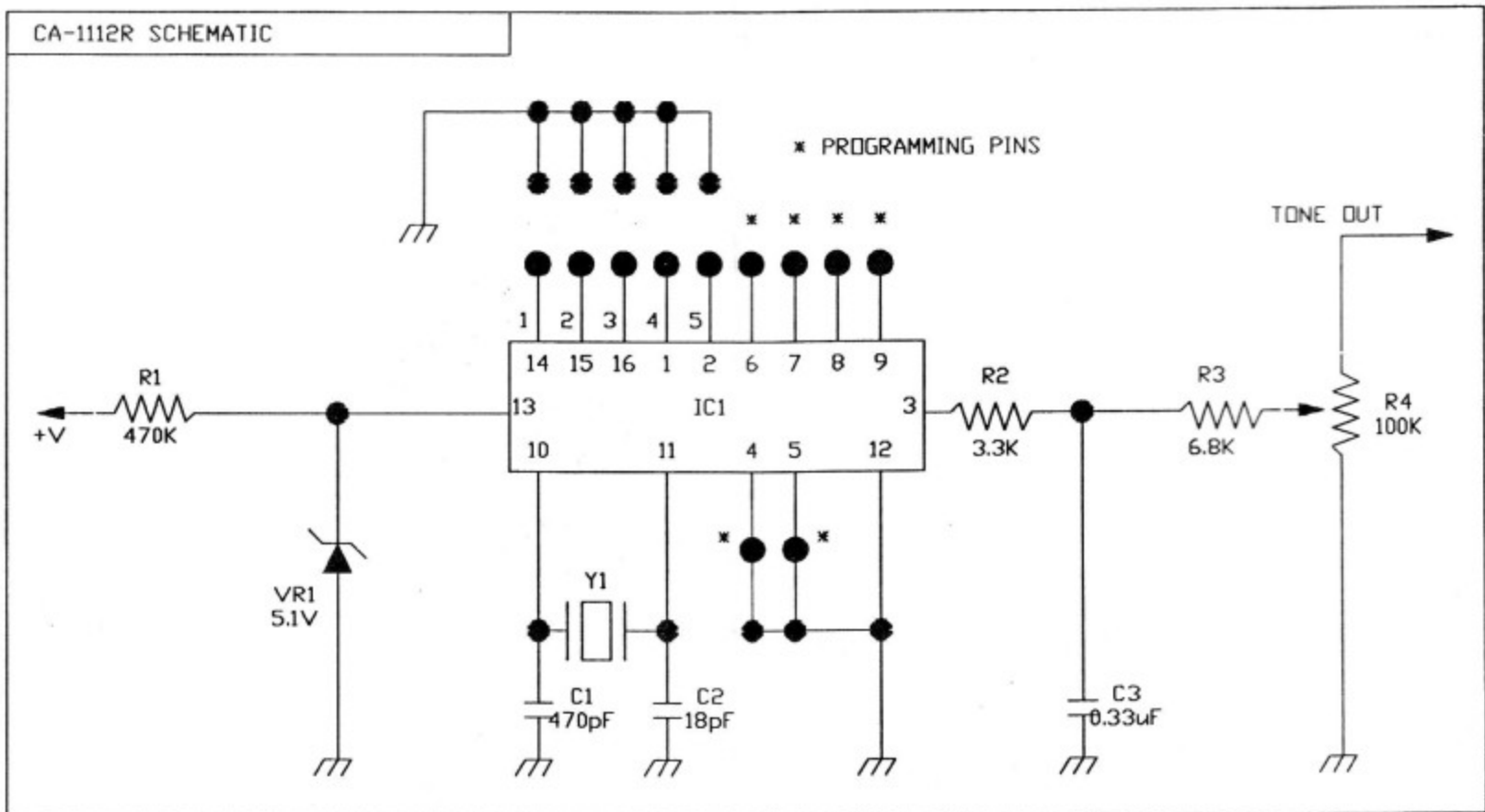
CA-1112R SCHEMATIC
