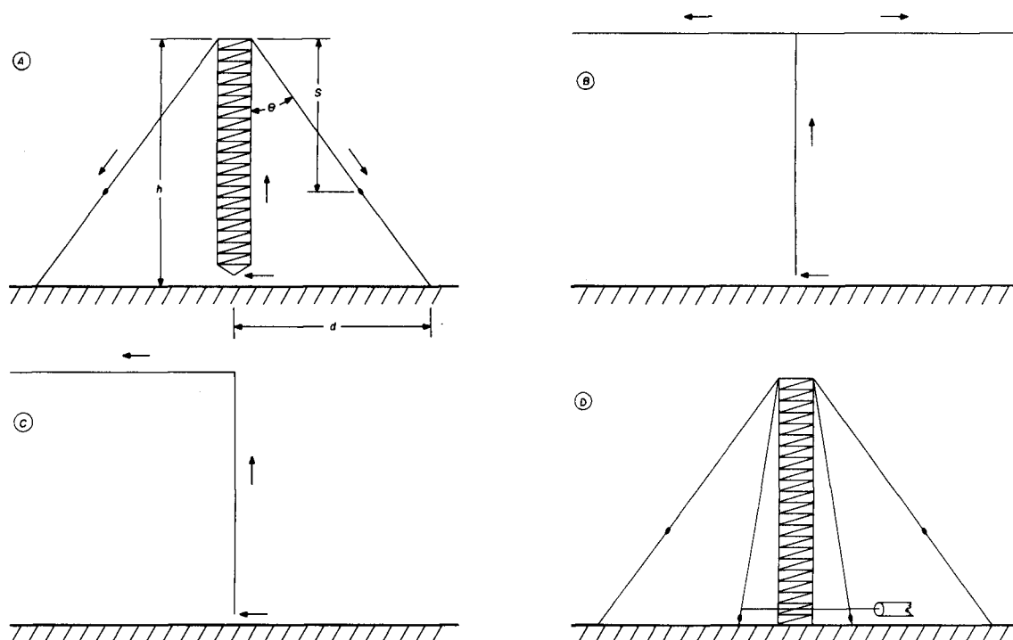
fig. 1. Wire antennas discussed in the text. A , the umbrella type top loaded vertical antenna, base-insulated tower (arrows illustrate the phasing of the current on the antenna). B , T-type top loaded vertical radiator (insulated base). C , L-type top loaded vertical radiator (insulated base), and D , folded umbrella antenna.
